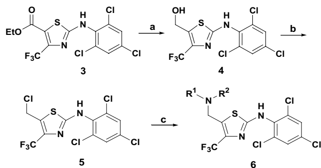
Scheme 1. Reagents and conditions: (a) DIBAL-H, THF, 0°C to rt, 2 h, 100%; (b) SOCl 2 , 85°C, 5 min, 91%; (c) R 1 R 2 NH, Et 3 N, diethyl ether, rt, 15 min, 50–95%.
